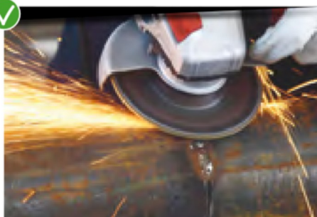
GRINDING OF CONVEX CURVED SURFACES
